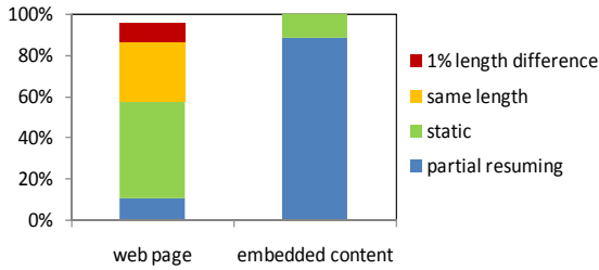
Fig. 10: Most web pages and all of their embedded content (among our top 100 pages) are supported by Resumption Agent
