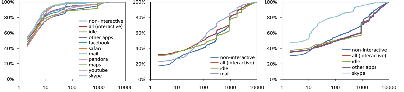
Fig. 5: CDF of TCP flow lifetimes (seconds), based on active application. (Left): web ports. (Center): email ports, (Right): other ports.
