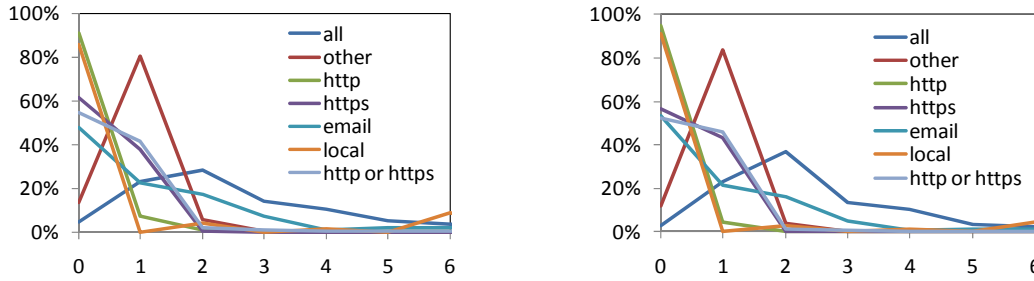
Fig. 2: We observed few concurrent TCP flows (Median = 2), and non-interactive and interactive usage were similar. Distribution of number of concurrent TCP flows for different TCP ports, average among all users. (Left: non-interactive sessions. Right: interactive sessions.)
