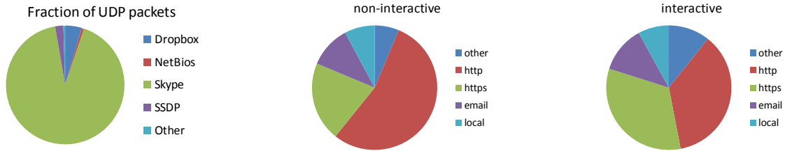
Fig. 1. Fraction of packets according to application for UDP packets (Left). Fraction of TCP flows for each application type (Center: non-interactive sessions. Right: interactive sessions, i.e. phone display was on).
