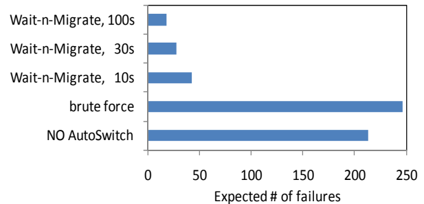
Fig. 14: AutoSwitch significantly reduces the expected number of disruptions in 1120 hours of interactive usage traces with Wi-Fi enabled, for different wait-time values
